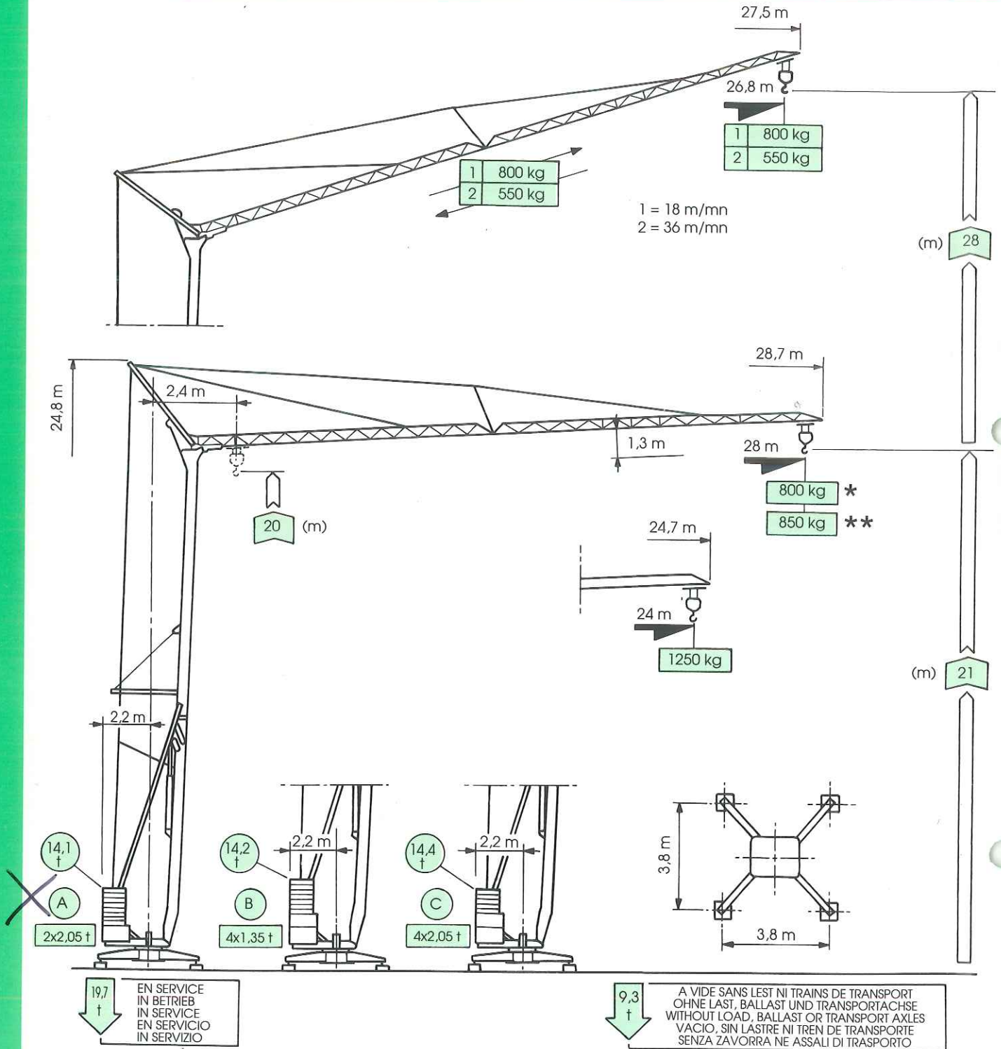
CHRONOFLASH 28 - 2500 kg
